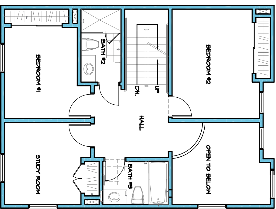
UNIT A SECOND FLOOR PLAN
