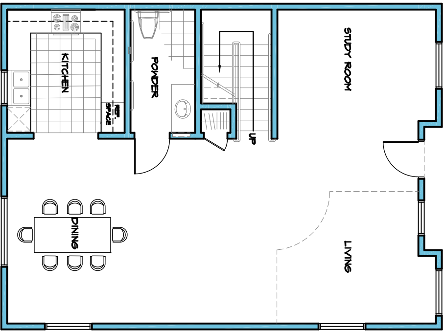
UNIT A FIRST FLOOR PLAN
